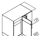
UESA Space filler for corner sink base unit ↳ 110/115/125 ↓ 75 ↙ 60
