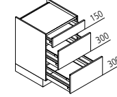
KUAK Hob base unit ↳ 60/80/90/100/120 ↓ 75 ↙ 60
