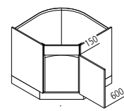
UES Corner sink base unit ↳ 90 ↓ 75 ↙ 60
