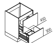
SAZ Sink base unit with waste separation system ↳ 60/80/90/100/120 ↓ 75 ↙ 60
