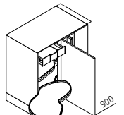
UELAD "LE MANS" spacefiller corner base unit ↳ 110/115/125 ↓ 90 ↘ 60
