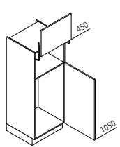
GKL Appliance housing with lift-up door for refrigerator / microwave / recess 880 mm ↓ 135/150 ↙ 60
