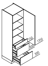
VAK Larder unit ↔ 30/40/45/50/60 ↓ 195/210/225 ↙ 60/50
