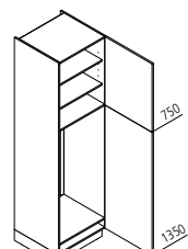
GK Appliance housing for refrigerator / recess 1225 mm ↔ 60 ↓ 195/210/225 ↙ 60
