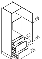
GKAK Appliance housing for refrigerator / recess 880 mm ↔ 60 ↓ 195/210/225 ↙ 60
