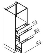
GBZ Appliance housing for oven or microwave ↔ 60 ↓ 135/150 ↙ 60
