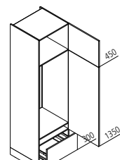
GKA Appliance housing for refrigerator / recess 1225 mm ↔ 60 ↓ 195/210/225 ↙ 60
