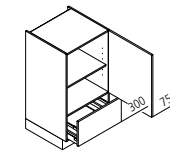
VA Larder unit ↔ 30/40/45/50/60 ↓ 105 ↖ 60/50
