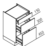
KUAK Hob base unit ↳ 60/80/90/100/120 ↓ 90 ↘ 60
