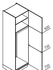
GK Appliance housing for refrigerator / recess 1440 mm ↔ 60 ↓ 195/210/225 ↙ 60
