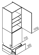
GGS A Appliance housing surround for dishwasher ← 60 ↓ 195/210/225 ↙ 60
