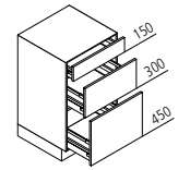
UAK Pull-out unit ↳ 30/40/45/50/60/80/90/100/120 ↓ 90 ↘ 60/50/39
