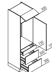
GKAK Appliance housing for refrigerator / recess 1025 mm ↔ 60 ↓ 195/210/225 ↙ 60
