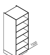
SR Open shelf units ↔ 20/25/30/35/40/45/50/55/60 ↓ 135/150 ↙ 60
