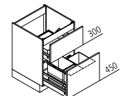
SUZ Sink base unit with waste separation system ↳ 60/80/90/100/120 ↓ 75 ↙ 60
