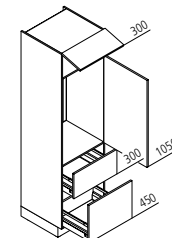
GKZ Appliance housing for refrigerator / recess 1025 mm ↔ 60 ↓ 195/210/225 ↙ 60
