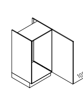
GK Appliance housing for refrigerator / recess 1025 mm ↔ 60 ↓ 105 ↖ 60
