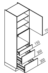
GBAK Appliance housing for oven / microwave ← 60 ↓ 195/210/225 ↙ 60
