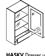
HASKV Dresser unit with glass door (depending on range) ↔ 45/50/60 ↓ 115 ↖ 35
