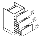
KAZ Hob base unit ↳ 60/80/90/100/120 ↓ 90 ↘ 60
