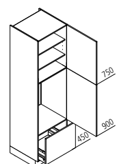
GKA Appliance housing for refrigerator / recess 880 mm ↔ 60 ↓ 195/210/225 ↙ 60
