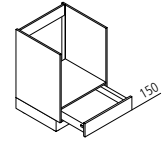
UHSK Cooker unit with drawer ↳ 60 ↓ 75 ↙ 60
