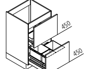
SUZ Sink base unit with waste separation system ↳ 60/80/90/100/120 ↓ 90 ↘ 60
