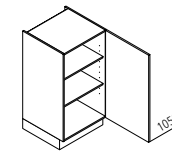
V Larder unit ↔ 30/40/45/50/60 ↓ 105 ↖ 60/50/35
