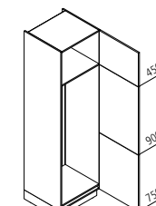
GKG Appliance housing for fridge/freezer combination / recess 1580 mm ↓ 195/210/225 ↙ 60
