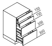
USA Drawer base unit ↳ 30/40/45/50/60/80/90/100/120 ↓ 90 ↘ 60/50/39
