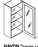
H AVDN Dresser unit with glass door DN ↔ 45/50/60 ↓ 115/130/145 ↖ 35
