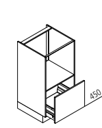
GBZ Appliance housing for oven or microwave ↔ 60 ↓ 105 ↖ 60
