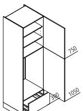
GKA Appliance housing for refrigerator / recess 1025 mm ↔ 60 ↓ 195/210/225 ↙ 60
