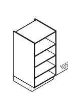
SR Open shelf units ↔ 20/25/30/40/45/50/60 ↓ 105 ↖ 60
