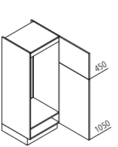
GKG Appliance housing for fridge/freezer combination / recess 1225 mm ↔ 60 ↓ 135/150 ↙ 60
