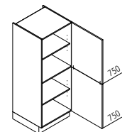
V Larder unit ↔ 30/40/45/50/60 ↓ 135/150 ↙ 60/50/35
