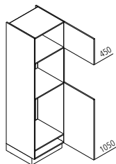
GKB Appliance housing for refrigerator and oven / recess 880 mm ← 60 ↓ 195/210/225 ↙ 60
