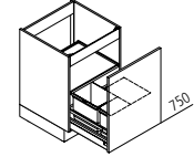
SABD Sink base unit with waste separation system ↳ 45/50/60 ↓ 75 ↙ 60
