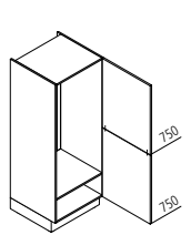
GK Appliance housing for refrigerator / recess 1225 mm ↔ 60 ↓ 135/150 ↙ 60
