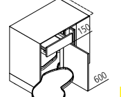
UELA Corner base unit ↳ 110/115/125 ↓ 75 ↙ 60
