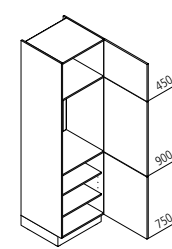
GK Appliance housing for refrigerator / recess 880 mm ↔ 60 ↓ 195/210/225 ↙ 60
