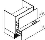
KUZ Hob base unit for use with aspiration hob ↳ 60/80/90/100/120 ↓ 75 ↘ 60
