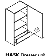
HASK Dresser unit ↔ 45/50/60 ↓ 115 ↖ 35
