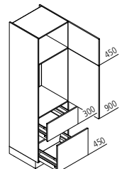
GKZ Appliance housing for refrigerator / recess 880 mm ↔ 60 ↓ 195/210/225 ↙ 60
