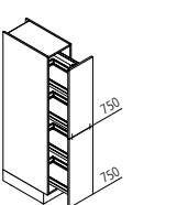
VVA Larder unit ↔ 30/40 ↓ 135/150 ↙ 60
