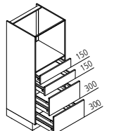
GBAK Appliance housing for oven or microwave ↔ 60 ↓ 135/150 ↙ 60
