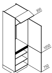
GK Appliance housing for refrigerator / recess 1025 mm ↔ 60 ↓ 195/210/225 ↙ 60
