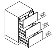
UAZI Pull-out unit ↳ 30/40/45/50/60/80/90/100/120 ↓ 90 ↘ 60/50/39
