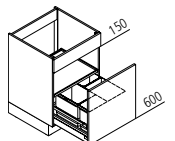
SAB Sink base unit with waste separation system ↳ 45/50/60/80/90/100/120 ↓ 75 ↙ 60
