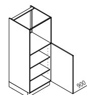
GB Appliance housing for oven or microwave ↔ 60 ↓ 135/150 ↙ 60
