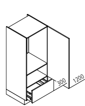
GKA Appliance housing for refrigerator / recess 880 mm ↔ 60 ↓ 135/150 ↙ 60
